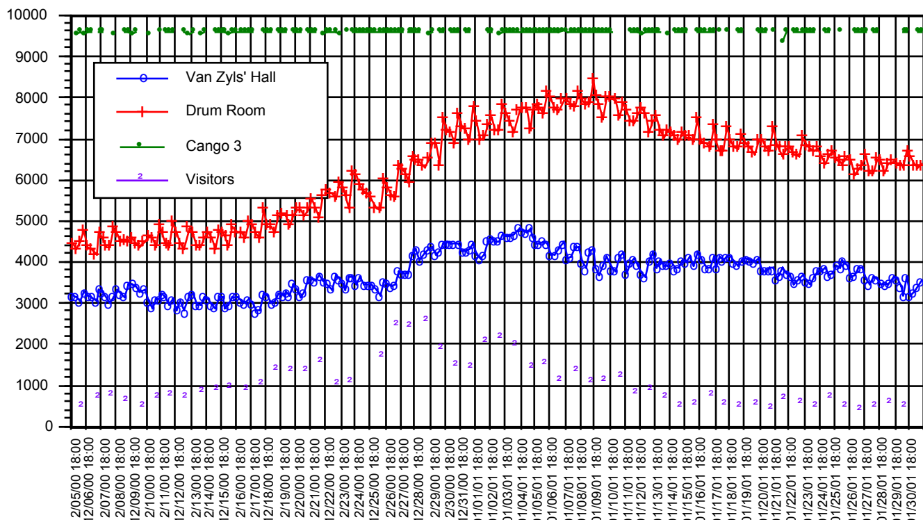
Fig. 3 - CO 2 concentrations (ppm) Congo Cave from December 5, 2000 to January 30, 2001. The daily number of visitors is also reported
